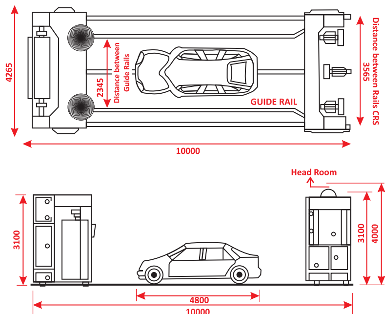
GENERAL LAYOUT OF KRE CAR WASH WITH DRYING UNIT
